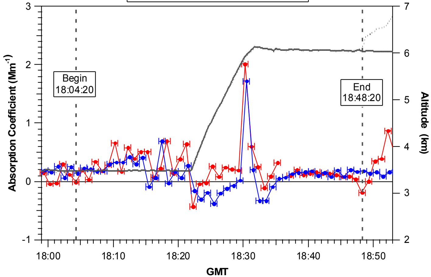
470 nm Total Absorption 04/17/2006 —●— DC-8 ABS R1 —●— C-130 ABS R2
