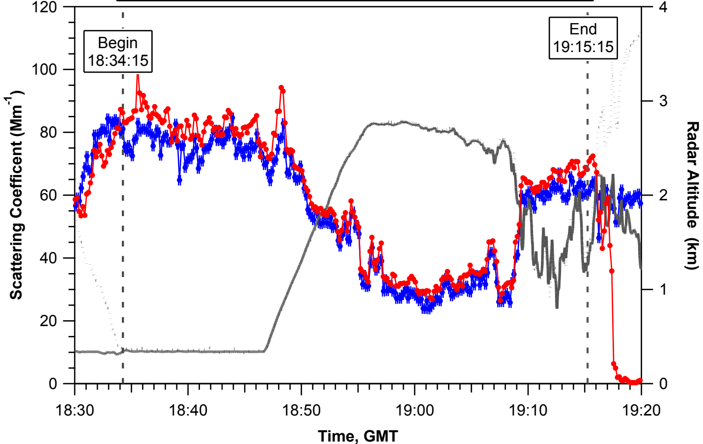
550 nm Total Scattering Comparison 03/19/2006 —●— DC-8 TSI R1 1/2LOD=0.35 —●— C-130 TSI R1 1/2LOD=0.35
